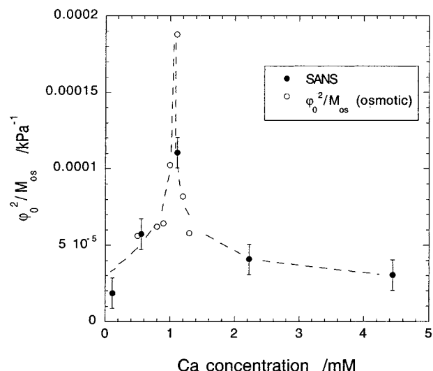
Figure 8. Comparison between the osmotic susceptibility \varphi_0^2/M_{os} determined from the macroscopic measurements (open circles) and the amplitude of the dynamic contribution of the SANS spectrum (filled circles). The latter data have been multiplied by the factor 3.8 \times 10^{-3} .
