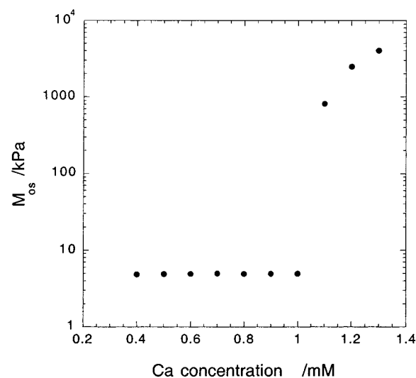
Figure 5. Dependence on \text{CaCl}_2 concentration of the longitudinal osmotic modulus M_{os} calculated from eq 5.
