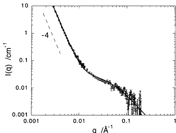
Figure 6. SANS intensity from sodium polyacrylate hydrogel in 40 mM NaCl solution containing 1.1 mM \text{CaCl}_2 . Note at low values of q the intensity varies nearly as q^{-4} , characteristic of scattering from a surface (see text).
