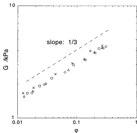
Figure 2. Measured values of the shear modulus G as a function of polymer volume fraction \phi in 40 mM NaCl solutions containing different amounts of \text{CaCl}_2 (O, 0 mM \text{CaCl}_2 ; \Delta , 0.2 mM \text{CaCl}_2 ; \square , 0.5 mM \text{CaCl}_2 ; \times , 0.8 mM \text{CaCl}_2 ).
