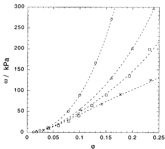
Figure 3. Dependence of the swelling pressure \omega on the polymer volume fraction \phi in 40 mM NaCl solutions containing different amounts of \text{CaCl}_2 (O, 0 mM \text{CaCl}_2 ; \Delta , 0.2 mM \text{CaCl}_2 ; \square , 0.5 mM \text{CaCl}_2 ; \times , 0.8 mM \text{CaCl}_2 ).
